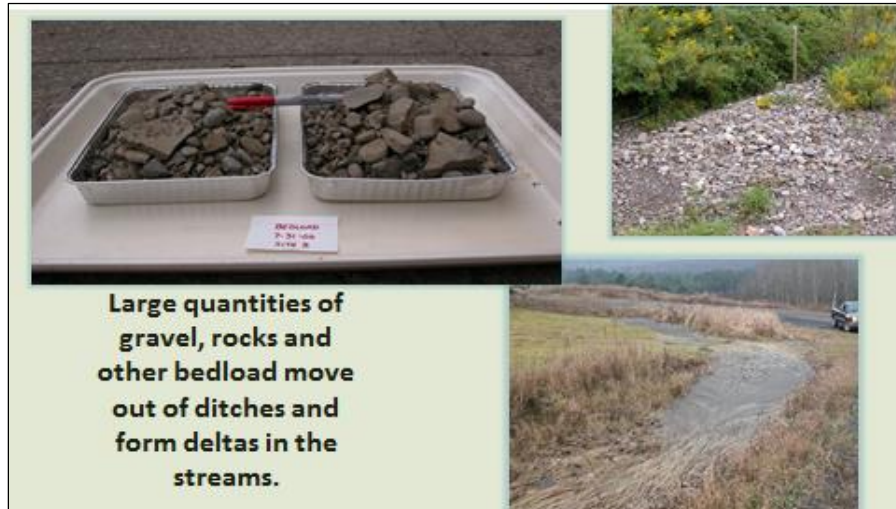
Samples of bedload gravel and rocks transported in a small rain event (top left) and the 3ft deep pile of bedload rock deposited in a single ditch during the 2006 flood in the Susquehanna River Basin (top right). Delta of bedload gravel deposited at bottom of ditch (lower) (Schneider 2014).
