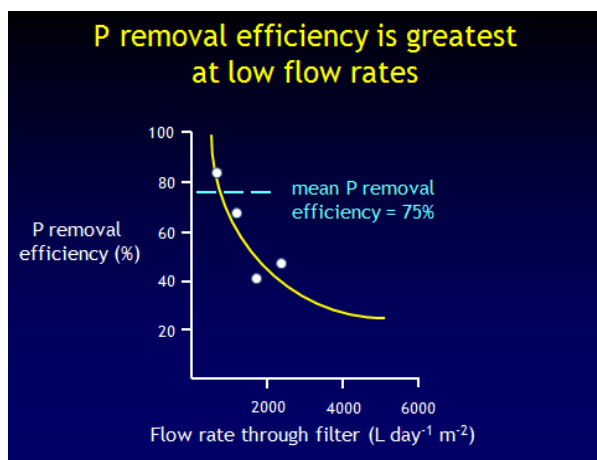
Filters for use in removing phosphorus (Bryant et al 2012).
