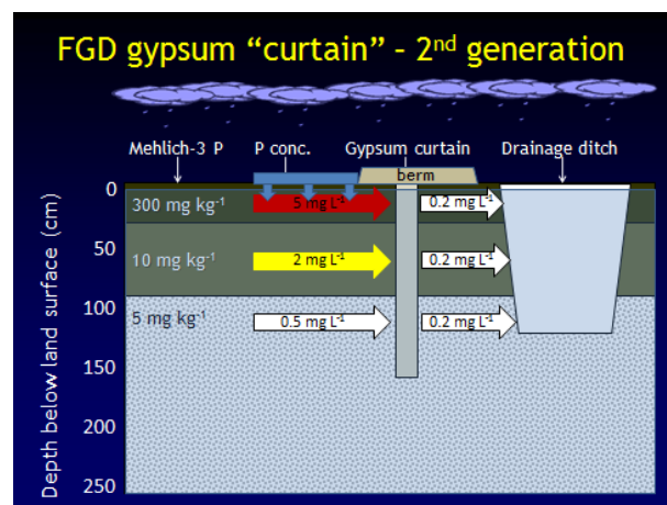
Filters for use in removing phosphorus (Bryant et al 2012).
